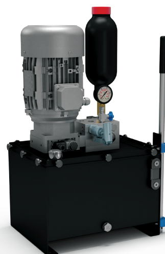
Serie 3 e 4 per Freni Negativi (N) e Positivi (P) Series 3 and 4 for Oil (P) and Spring Actuated Brakes (N)
